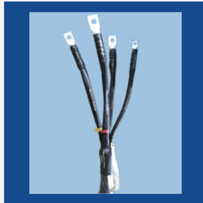
Low Voltage Heat Shrinkable Termination
